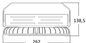
ALUMAX/N-L-100W
