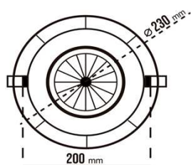
D-LED-IP65-25W-2300lm/840
