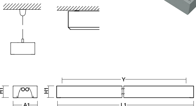
MOUNTING
