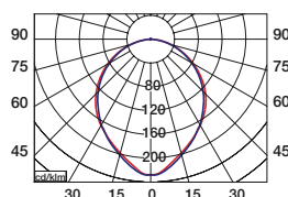
MN/PRISMA 2x36W
