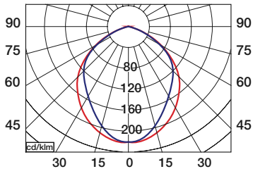
DTM-IP44-195 1x13 W.
