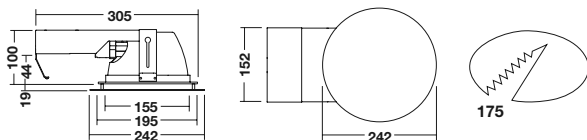
Mounting
